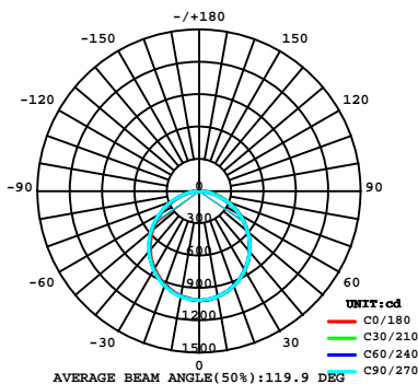
Photometric Diagram
